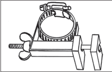
30010 - 1 Clamp Accessory
